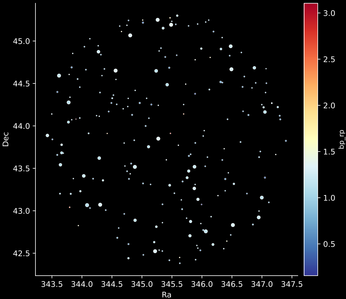
APOGEE DR17 Field: [069+45_MGA] Stars: 212
