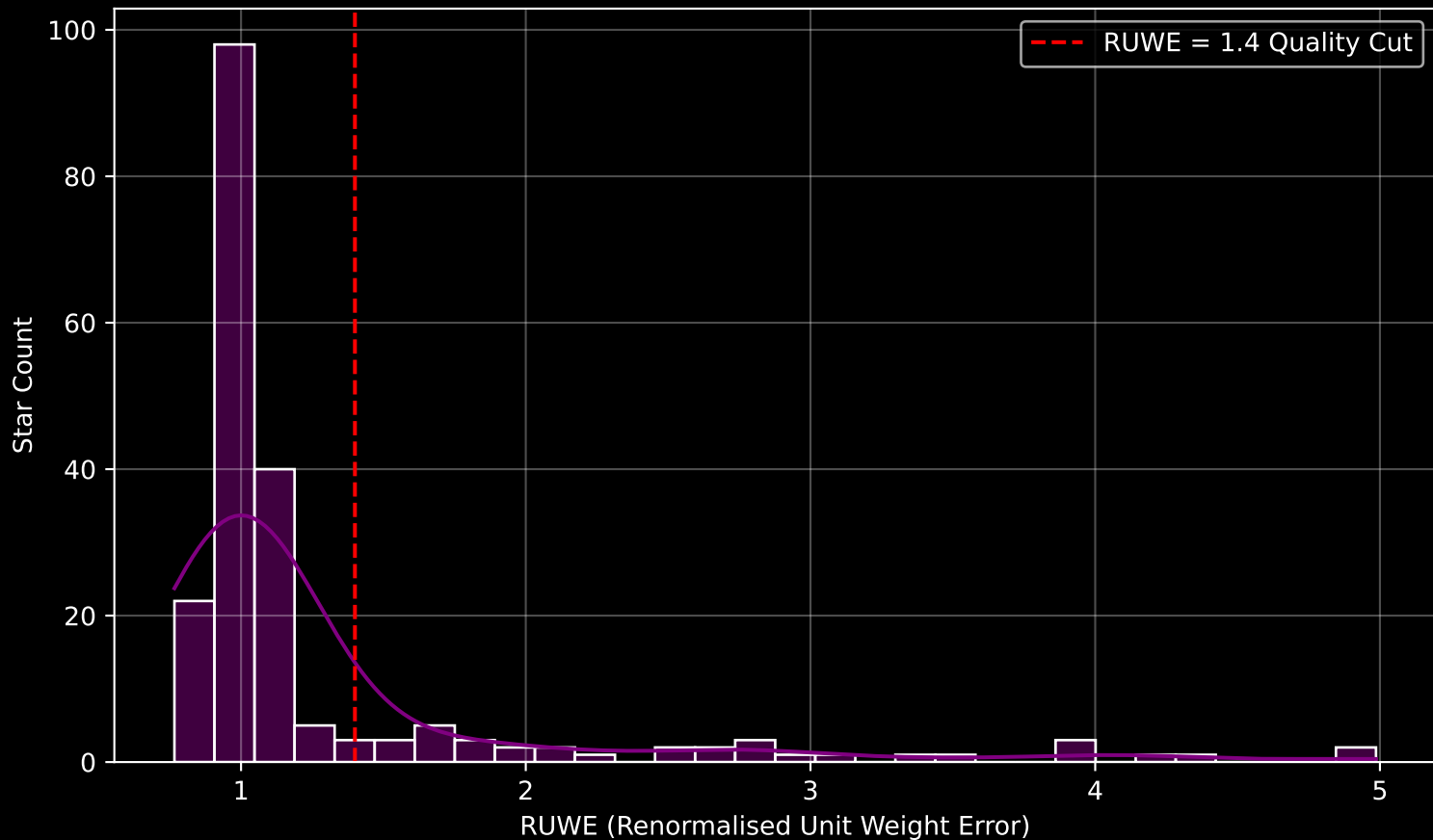
GAPOGEE DR17 Field [069+45_MGA] RUWE Distribution (n= 202)
