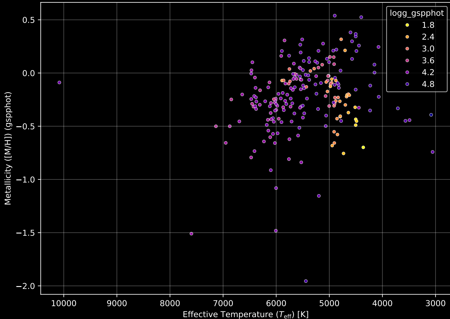
APOGEE DR17 Field: [069+45_MGA] Stellar Population Parameters (n= 212)
