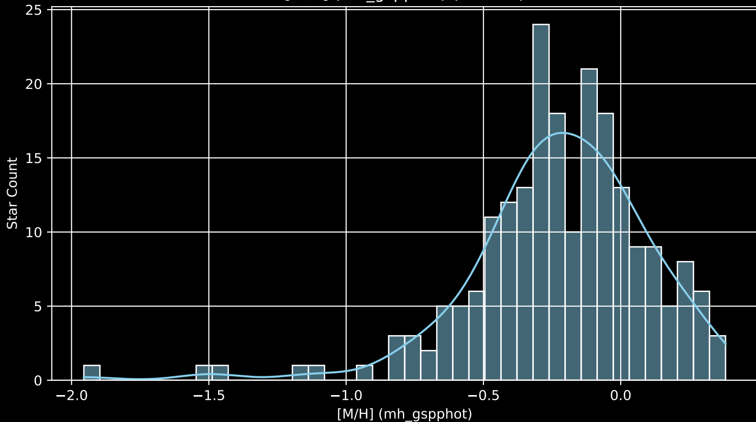
APOGEE DR17 Field: [069+45_MGA [M/H] (mh_gspphot) (n= 210)
