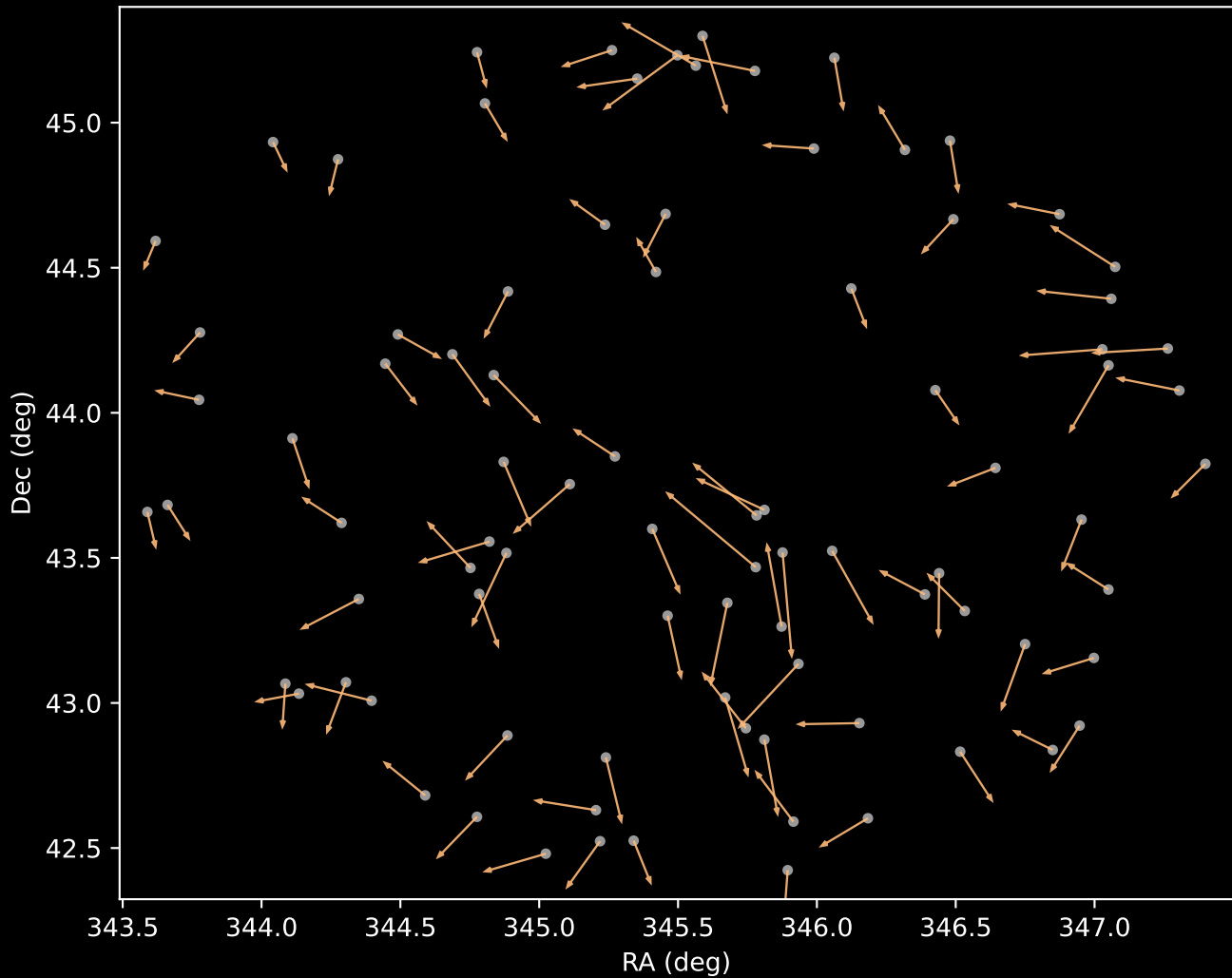
APOGEE DR17 Cluster 3 Proper Motion Vectors (n=88)
