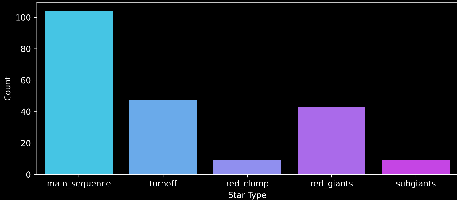
APOGEE DR17 Field: [069+45_MGA] Count plot of Star Type
