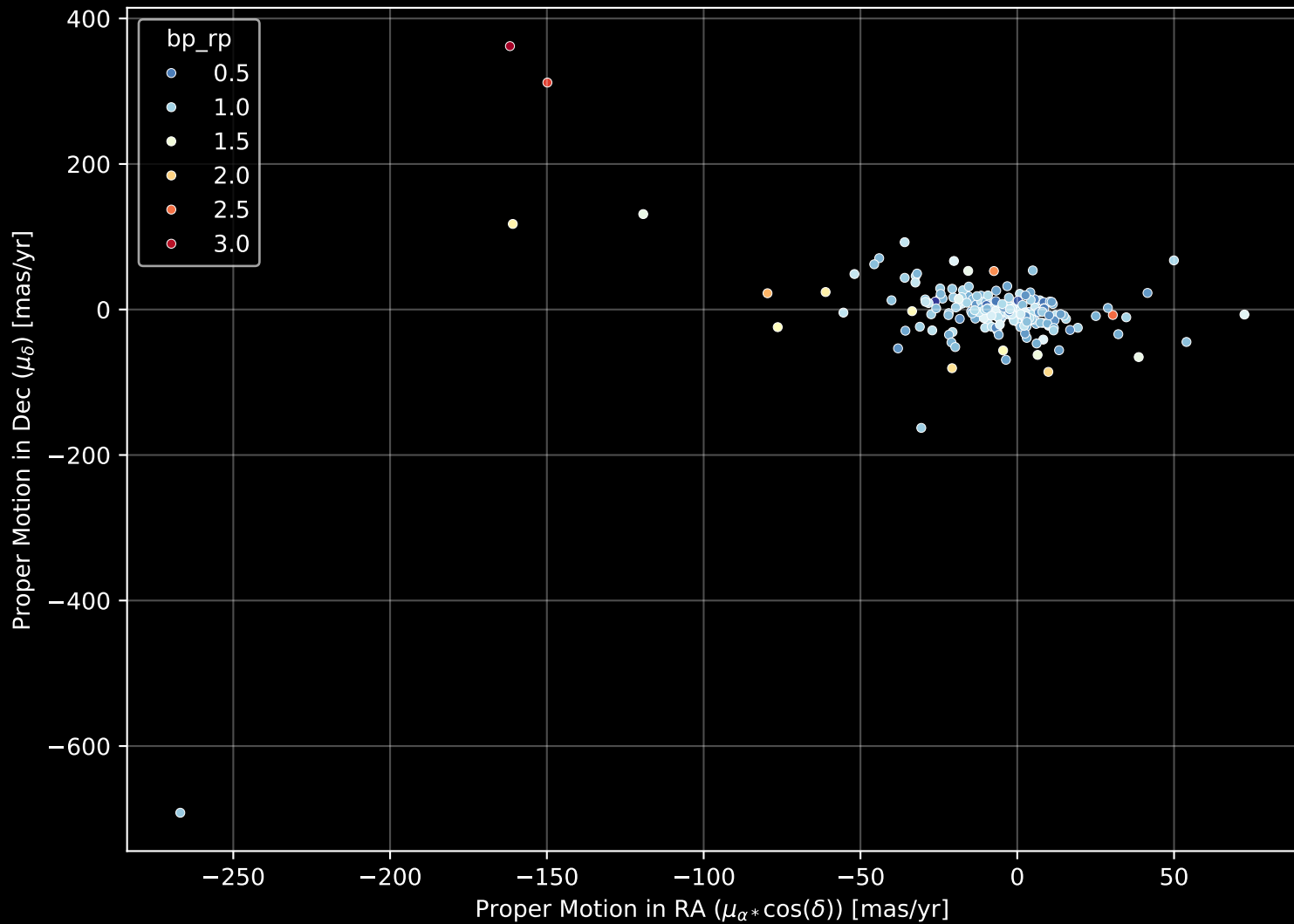
APOGEE DR17 Field: [069+45_MGA] Proper Motion Diagram (n= 212)
