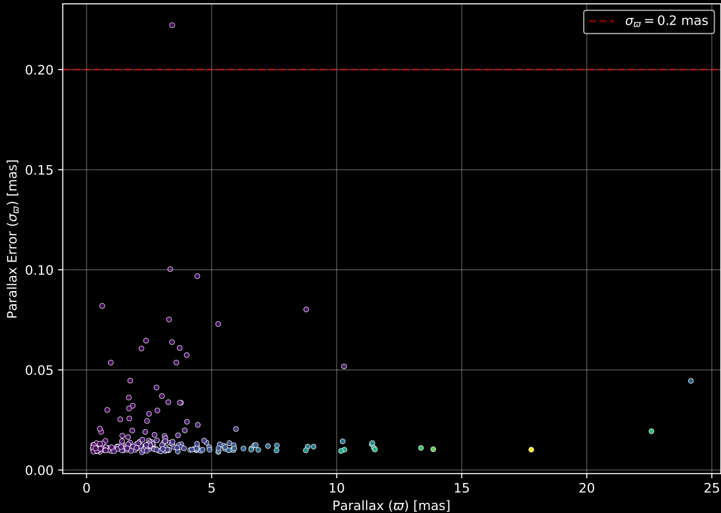
APOGEE DR17 Field: [069+45_MGA] Parallax Quality (n= 212)
